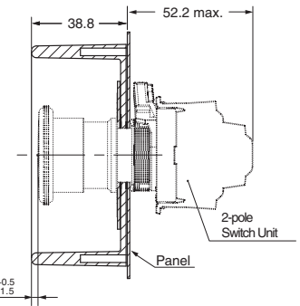
Push-in Plus Terminal Block Type Mounting a 2-pole Switch Unit
