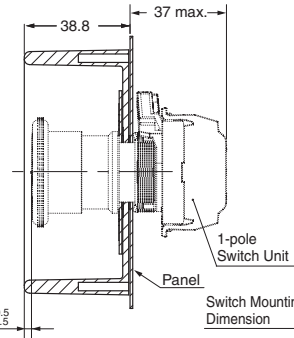
Push-in Plus Terminal Block Type Mounting a 1-pole Switch Unit
