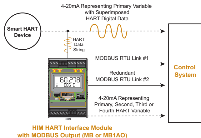
Figure 3. The HIM converts the HART digital protocol to MODBUS RTU (with MB or MBAO1 output type).
