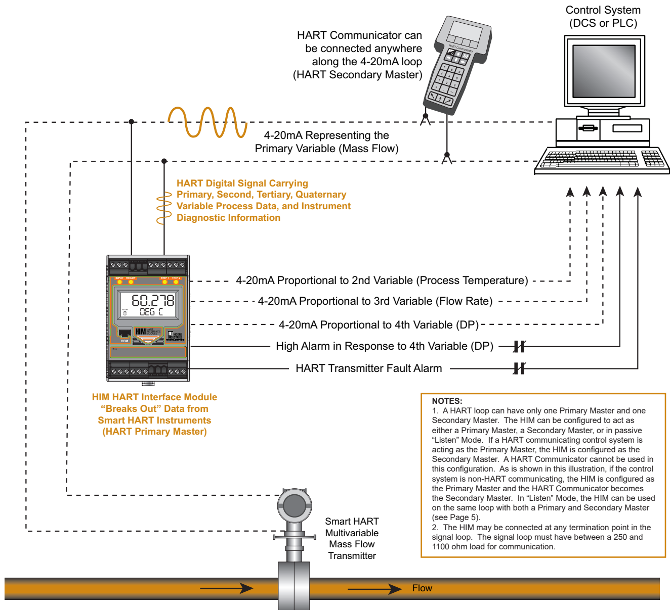
Figure 1. The HIM converts HART digital data to 4-20mA values proportional to a multivariable transmitter's primary, second, third or fourth variables. Its alarm trip outputs warn of unwanted high/low process conditions or of instrument diagnostic problems.
